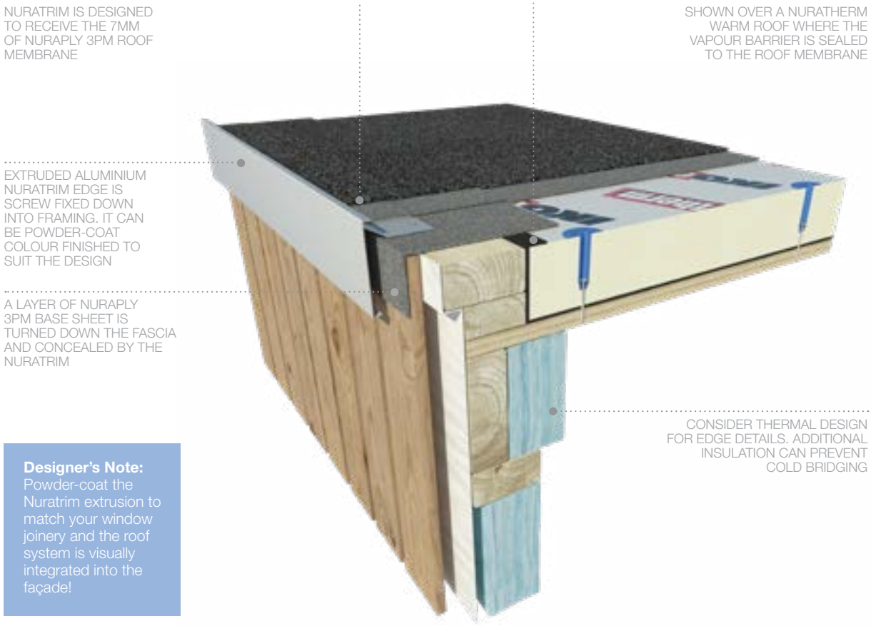
» Figure 17: NURATRIMS. MECHANICALLY FIXED EDGING SYSTEM FOR RESISTING DYNAMIC WIND FORCES. DETAIL SHOWN WITH A NURATHERM WARM ROOF
