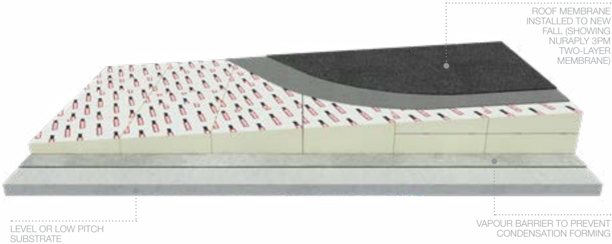
» Figure 08: DIAGRAM OF TAPERED PIR INSULATION LAYOUT
