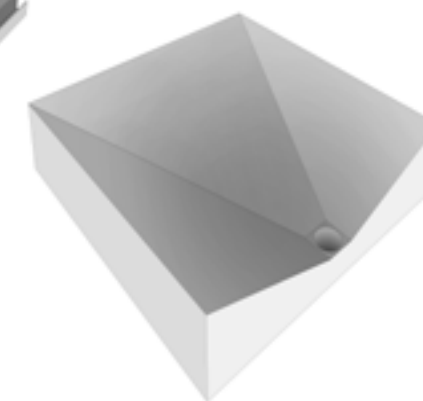
» Figure 12: VALLEY FALLS TO SIDE OUTLET
