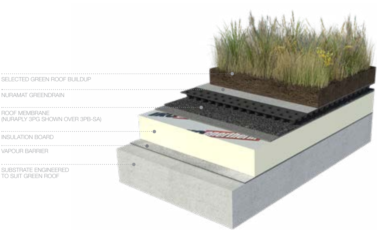
» Figure 01: GREEN ROOF SYSTEM. TYPICAL BUILDUP OF SEMI-INTENSIVE GREEN ROOF OVER NURAPLY 3PG MEMBRANE AND NURATHERM WARM ROOF
