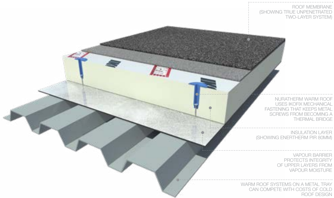
» Figure 04: NURATHERM WARM ROOF. DIAGRAM SHOWING CONTINUOUS INSULATION OF WARM ROOF DESIGN
