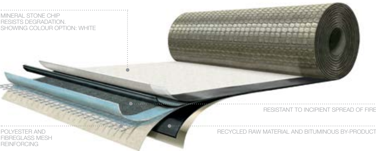
» Figure 06: MODERN MEMBRANE. THE QUALITY OF MODERN NURAPLY 3PM TORCH-ON IS THE RESULT OF A SOPHISTICATED MANUFACTURING PROCESS
