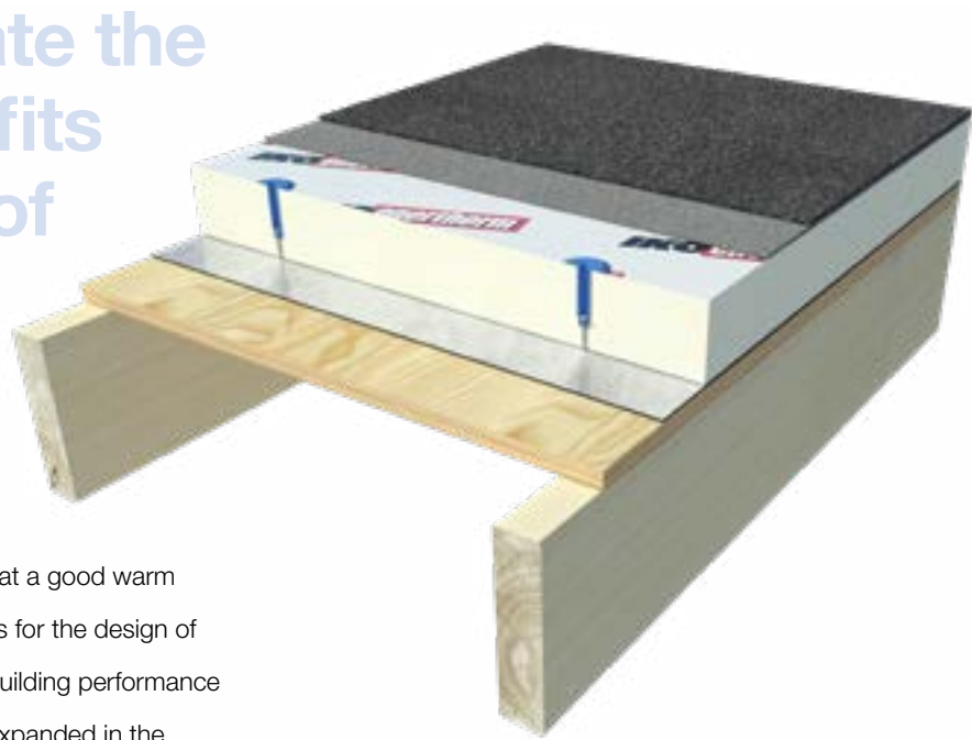
» Figure 05: TYPICAL WARM ROOF WITH CONTINUOUS INSULATION
