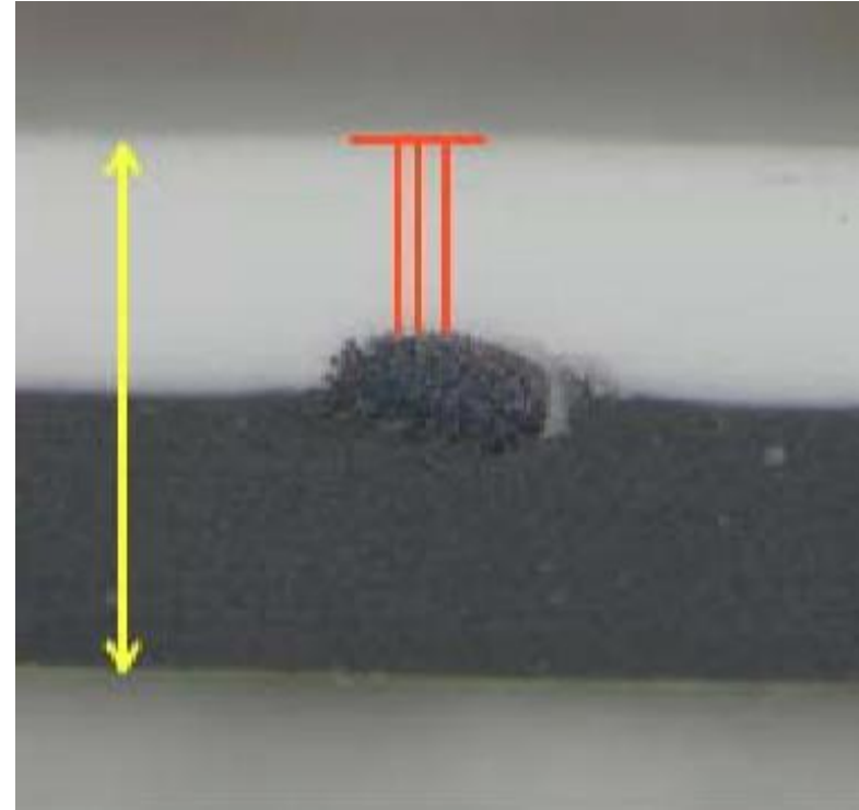
Difference between total thickness (yellow arrow) and thickness above scrim (orange lines)
