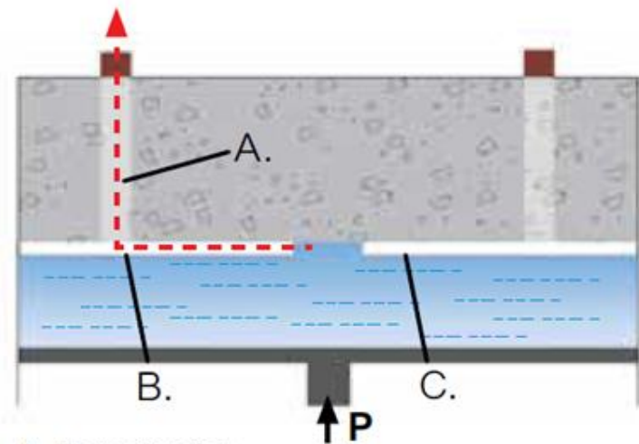
A. Flow of water B. Traditional membrane C. Preprufe® membrane
