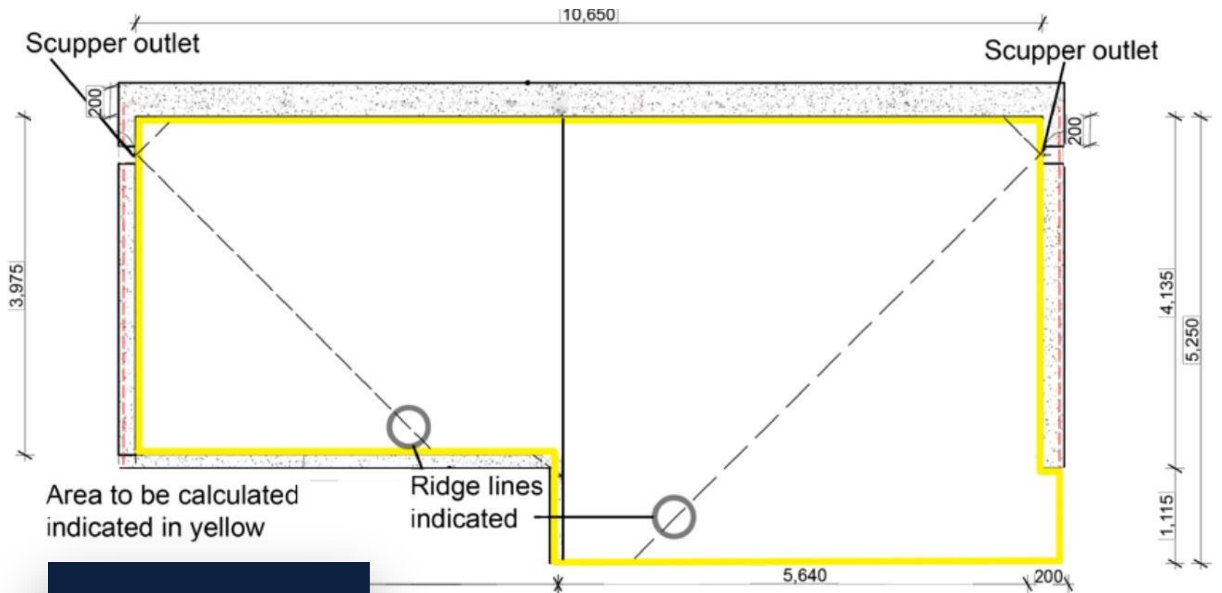
Basic Roof Plan
